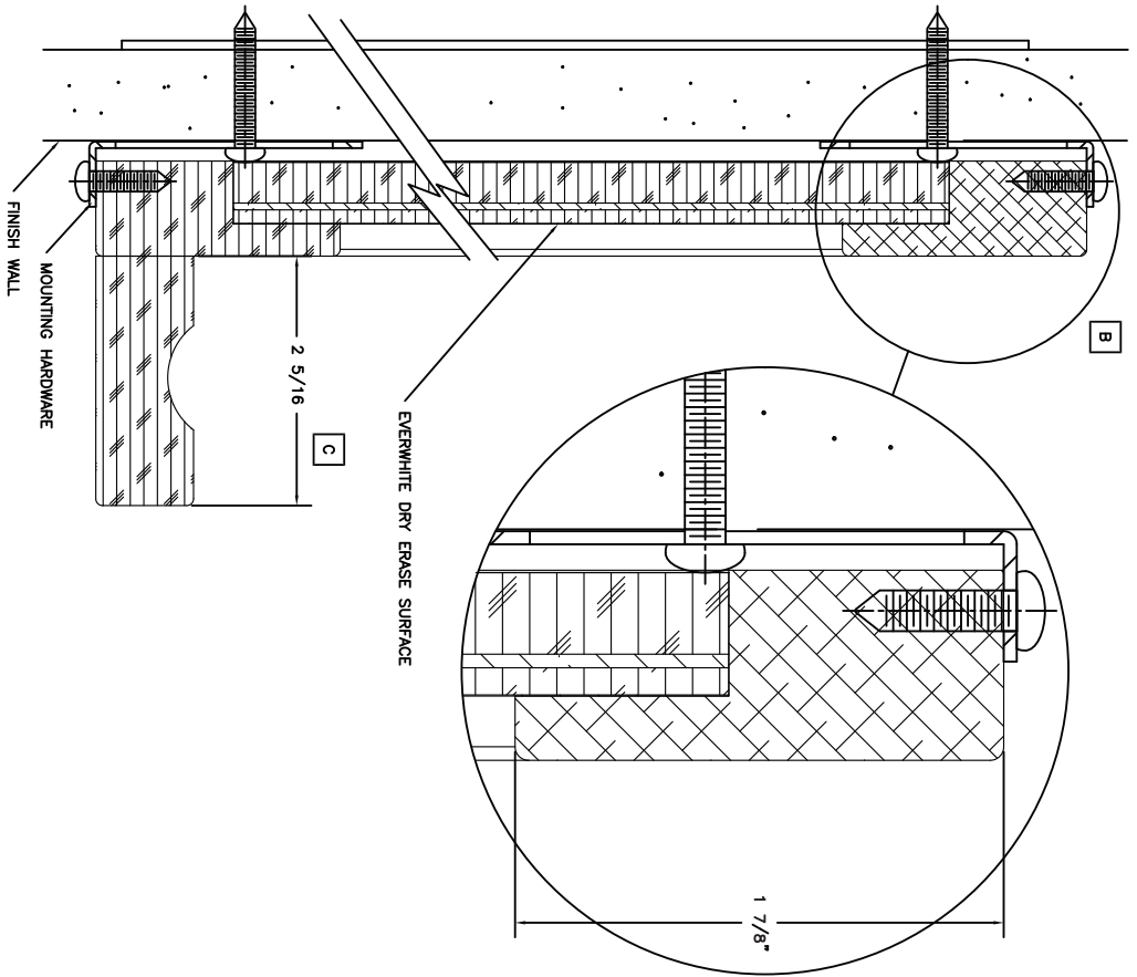
VERTICAL SECTIONS
