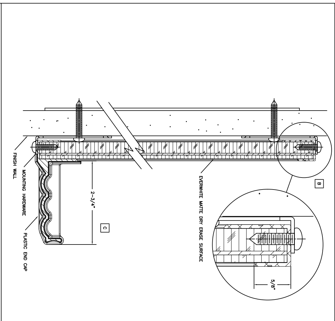
VERTICAL SECTIONS
