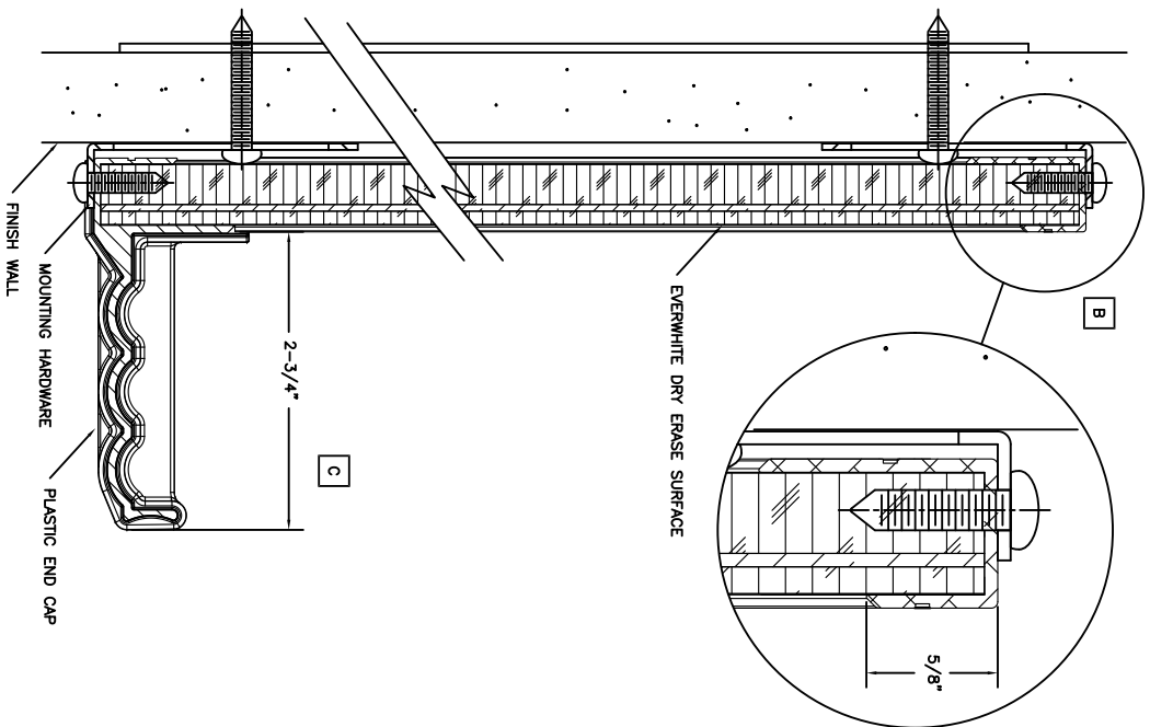
VERTICAL SECTIONS
