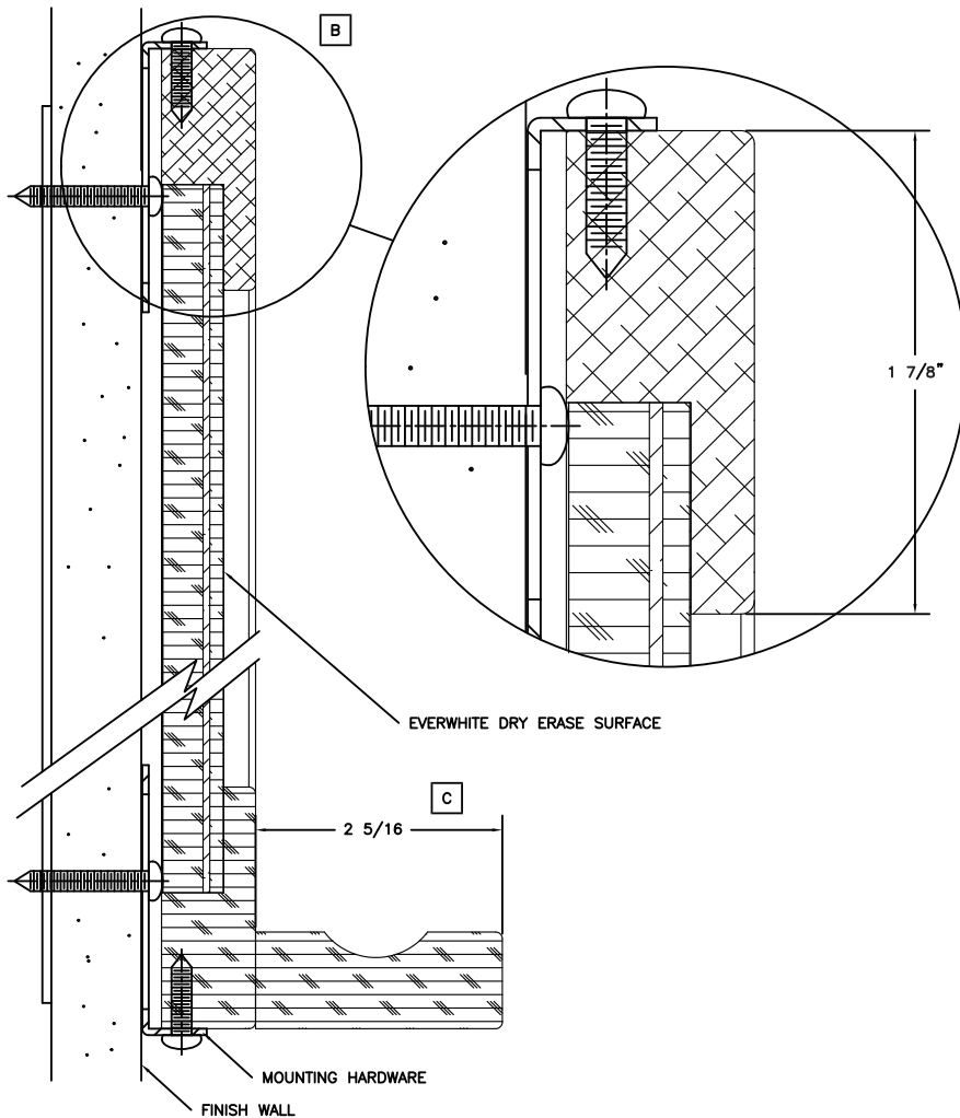
VERTICAL SECTIONS
