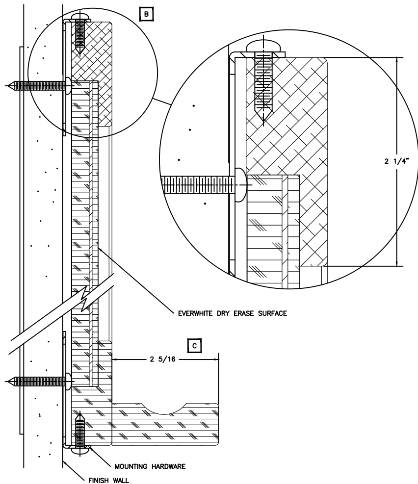
VERTICAL SECTIONS
